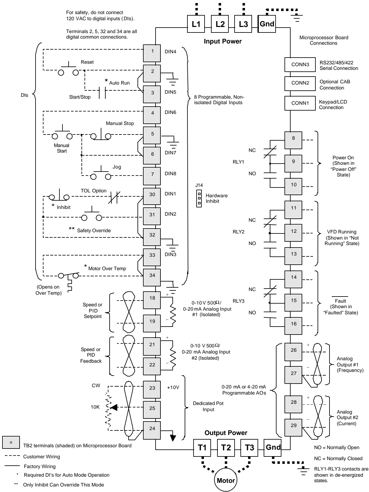
Figure 0-1. Typical 454 GT Control Connection Diagram (Based on a Standard SOP File) (Consult "As-Built" Drawings for Order-specific Wiring Configurations)
